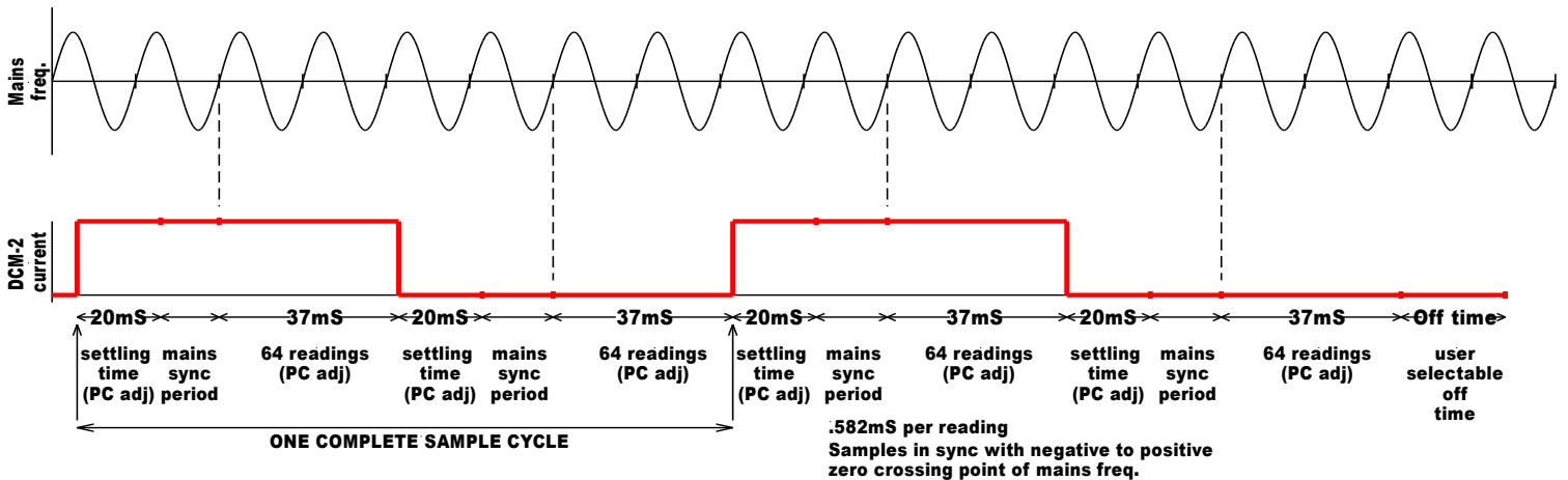
Figure 7 Free running mode.
