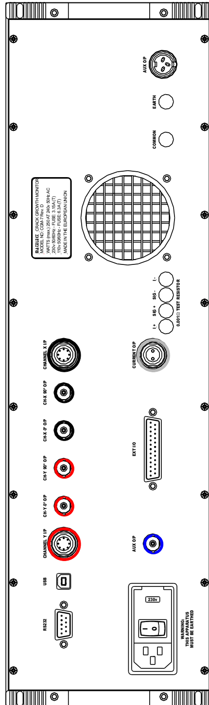
Fig 6. Rear Panel of the CGM7
