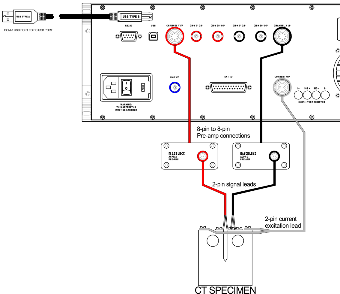
Fig 3. Block diagram of basic CGM7 system.
