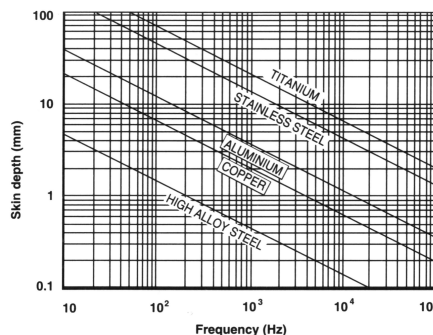
Fig 2. Skin depth v frequency for various materials.
