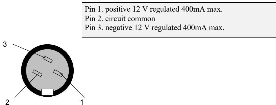
Fig 10 Auxiliary output socket
